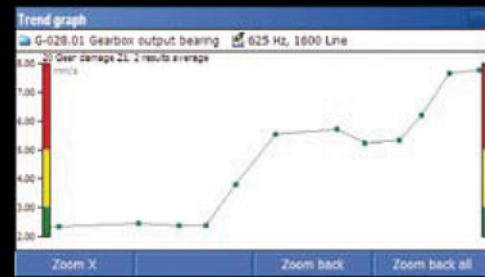
EVAM - trend evaluation
