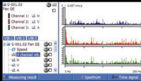
Tri-axial vibration measurements
