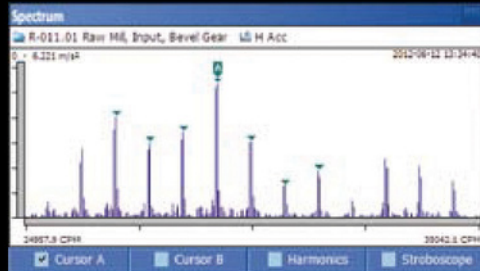
Gear box spectrum with sidebands
