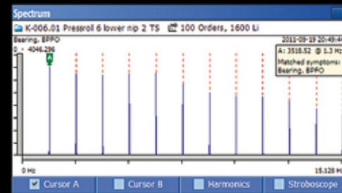
BPFO symptom in SPM HD spectrum
