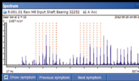
Spectrum with gear symptom
