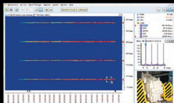
Coloured Spectrum Overview
