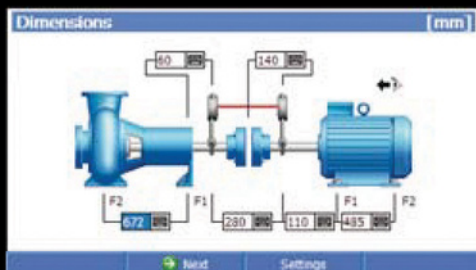
Laser shaft alignment
