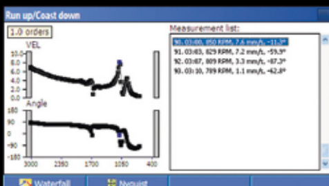
Run up - coast down measurements
